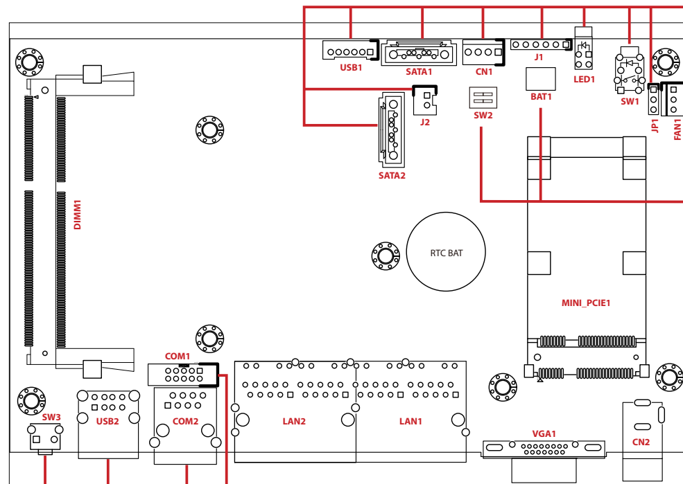
SW3: HW RESET BUTTON USB2: USB Port
